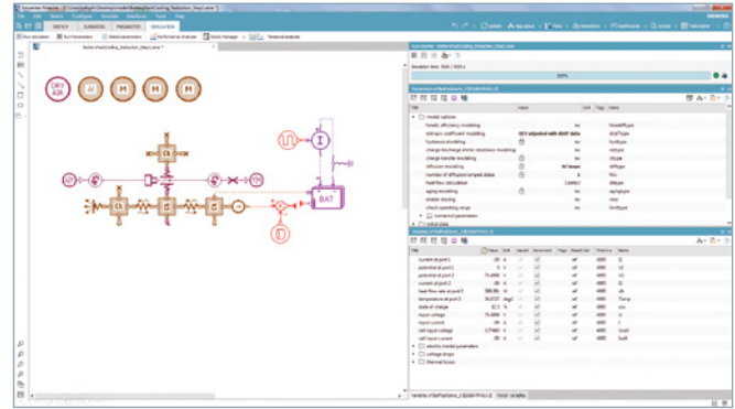
Figure 2: Simcenter Amesim battery model
