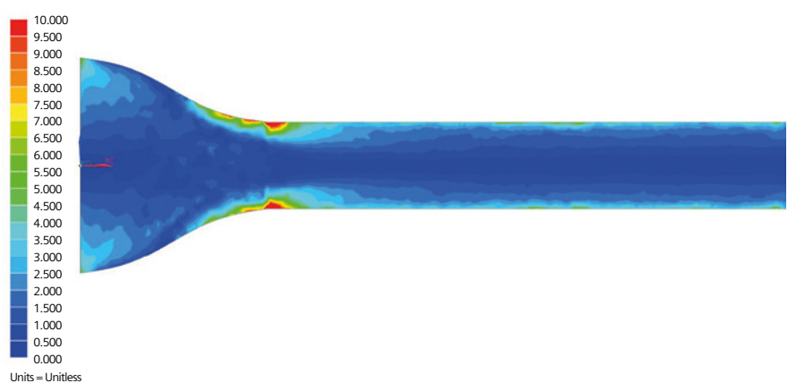
Figure 6: CFD simulation using Simcenter 3D Flow and Simcenter 3D Thermal was used to optimize the geometry of the wind tunnel asa hydraulik built at its headquarters in Vienna, Austria
