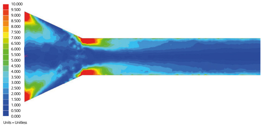
Kontraktion_stp_fem1_sim1: Solution 2 Result Load Case 1, Static Step 1 Vorticity - Element-Nodal, Unaveraged, Magnitude Min: 0.04, Max: 34.20, Units = Unitless
