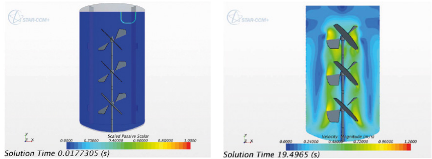
Figure 2: Simcenter STAR-CCM+ simulations of a triple low-shear impeller blender used to simulate the operation of full-scale bioreactor units
