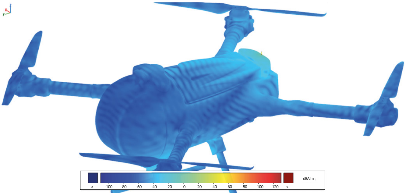
Figure 3: Induced Currents on a Colibri Drone
