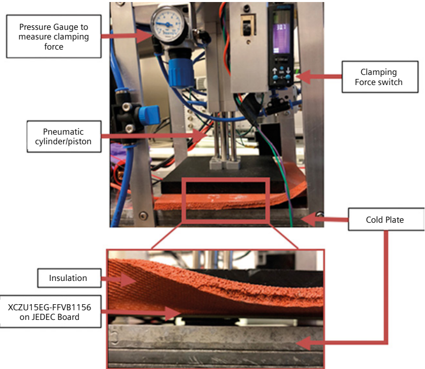
Figure 2: Measurement Fixture
