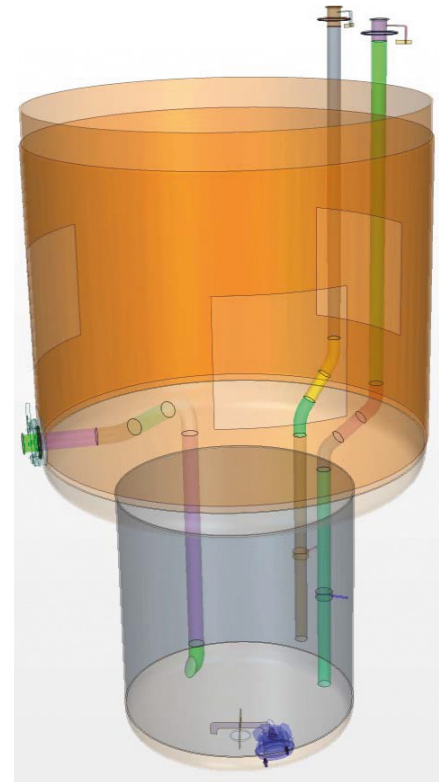
Figure 5: “Stepped volume” configuration used to manage batch geometry as product is concentrated in filtration applications
