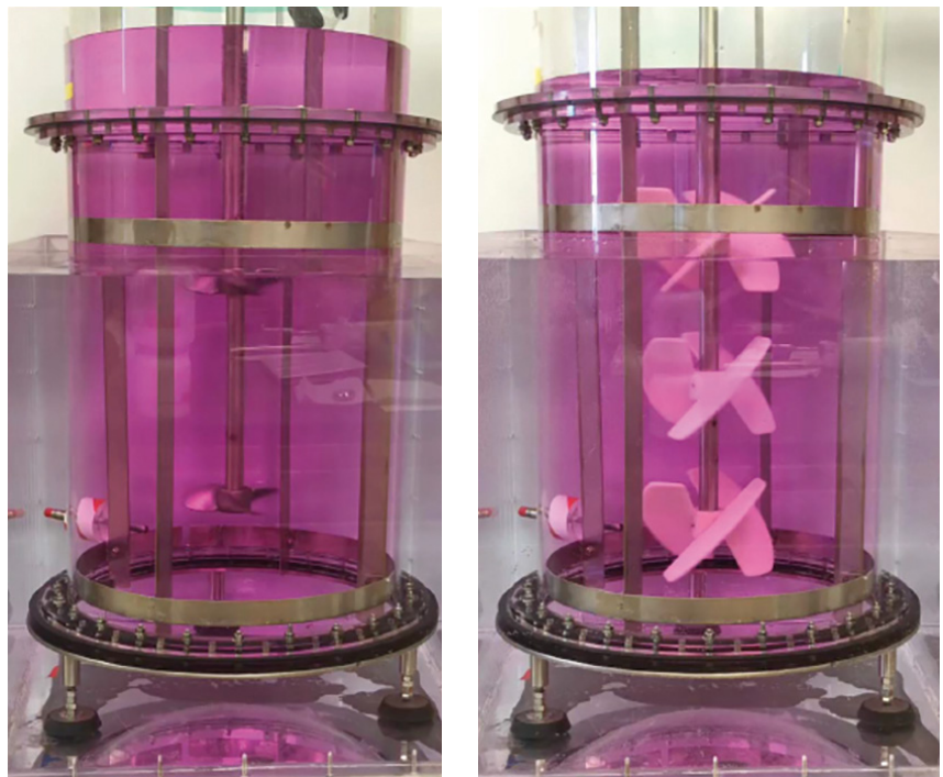
Figure 1: Experimental setups used for small-scale model testing of impeller configurations
