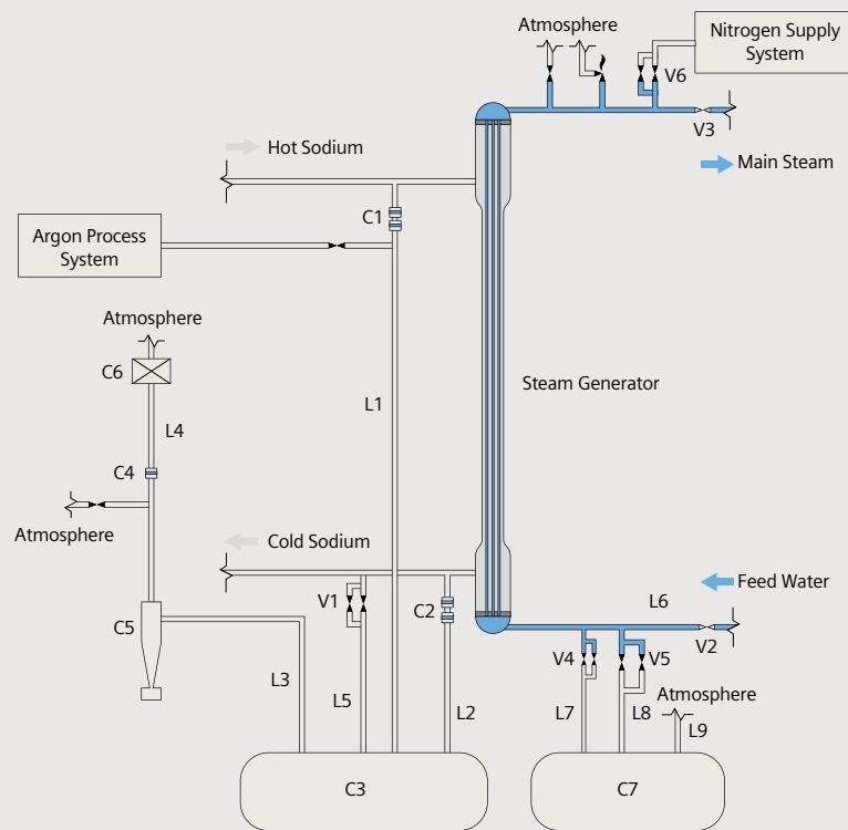
Figure 1. Schematic diagram of a SWRPRS. C1: Hot leg rupture disk, C2: Cold leg rupture disk, C3: Sodium dump tank, C4: Back pressure rupture disk, C5: Gas-liquid separator, C6: Hydrogen igniter, C7: Water dump tank. L1: Hot leg sodium dump line, L2: Cold leg sodium dump line, L3: Gas-liquid separator connection line, L4: Back pressure rupture disk gas vent line, L5: Cold leg sodium dump line, L6: Feedwater supply line, L7: Small diameter SG water dump line, L8: Large diameter SG water dump line, L9: WDT gas vent line. V1: Cold leg sodium dump line isolation valve, V2: Feed water isolation line valve, V3: Main steam line isolation valve, V4: Small diameter SG water dump line isolation valve, V5: Large diameter SG water dump line isolation valve, V6: Nitrogen supply line isolation valve
